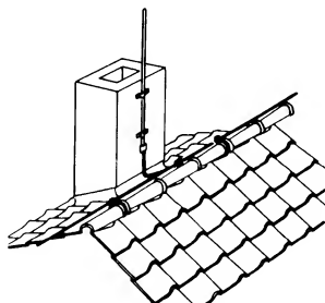
⑧ Chimneys with lightning conductor connected to the ridge conductor
